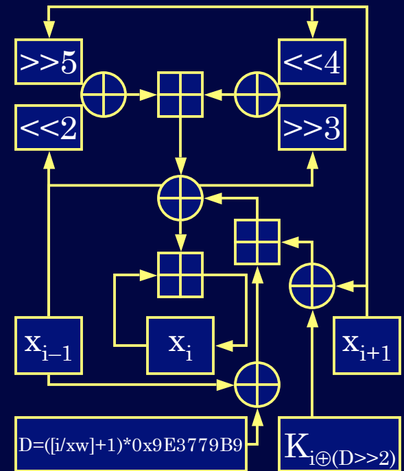
XXTEA: 10/21
