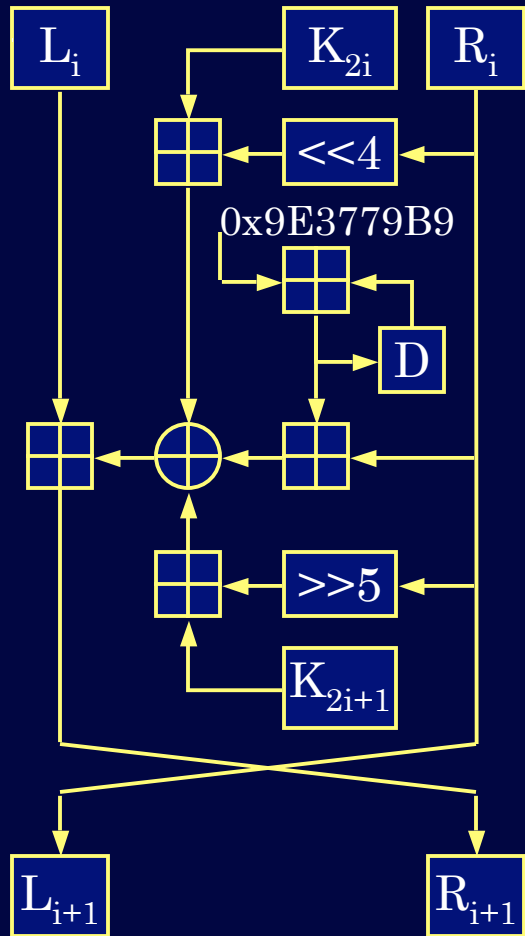
TEA: 10/∞
